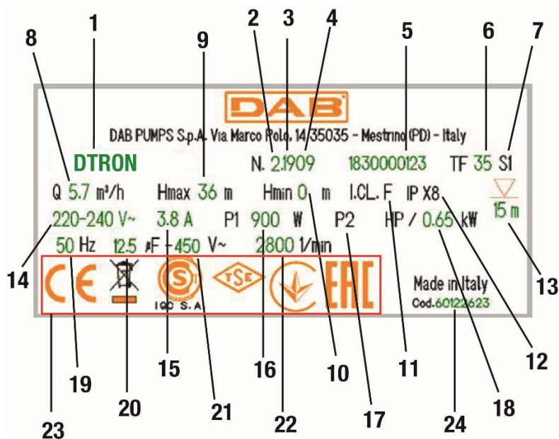
Fig.4 Data plate
